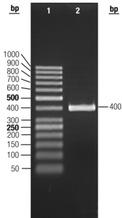
Fig.1. Analysis on agarose gel.
